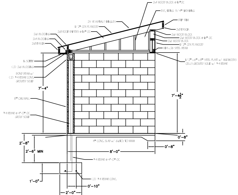
TYP. SECTION THRU PROPOSED DUGOUTS SCALE: 3/4"=1'-0"
